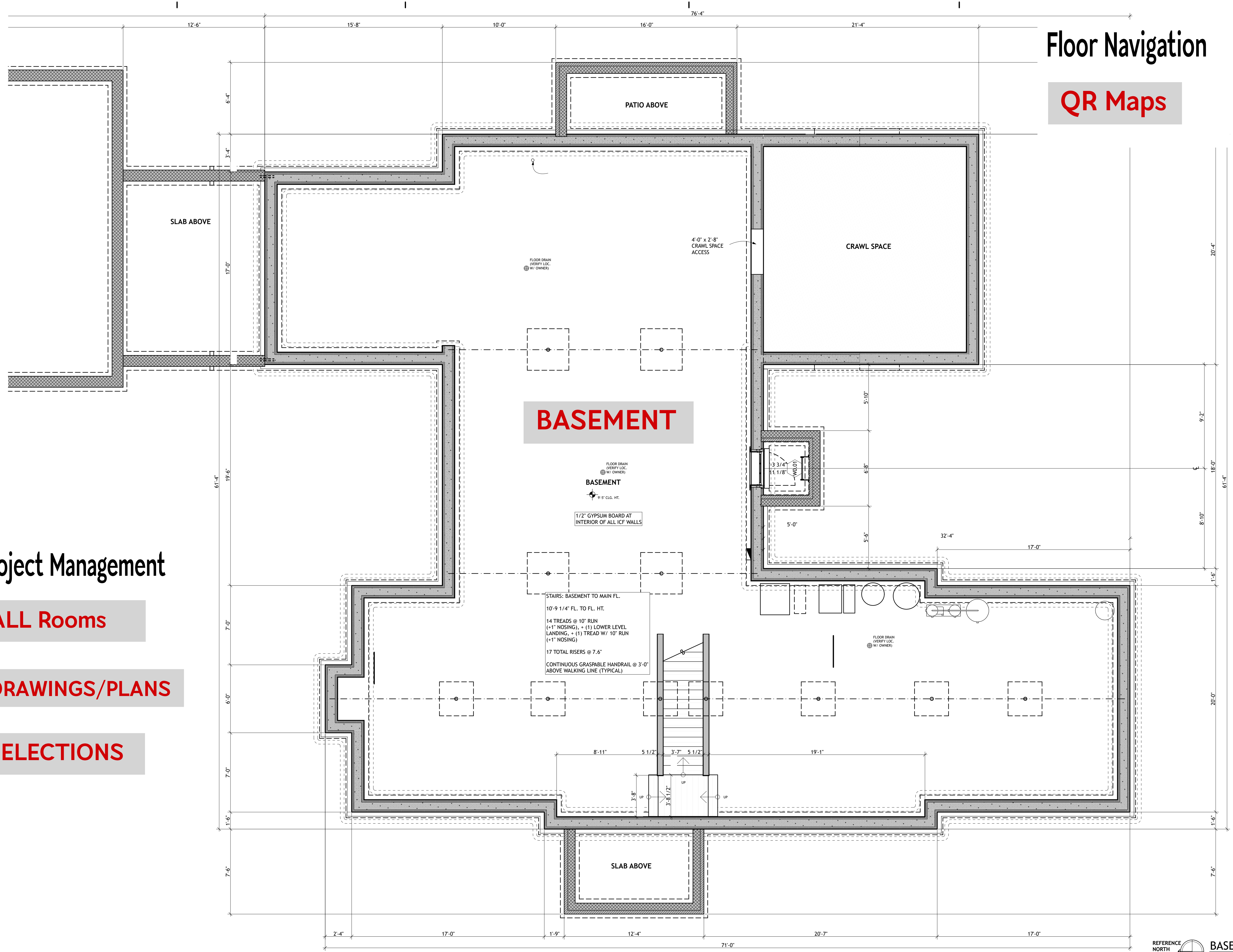
REFERENCE NORTH BASEMENT FLOOR PLAN 1/4" = 1'-0"
